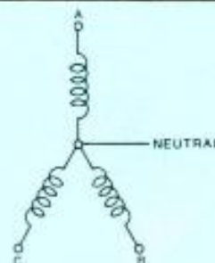
Figure 2. 3-phase WYE distribution transformer.
